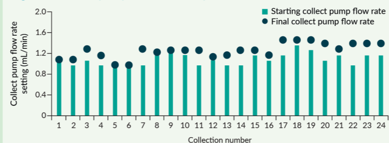
Figure 3. Collect pump flow rate comparison.
